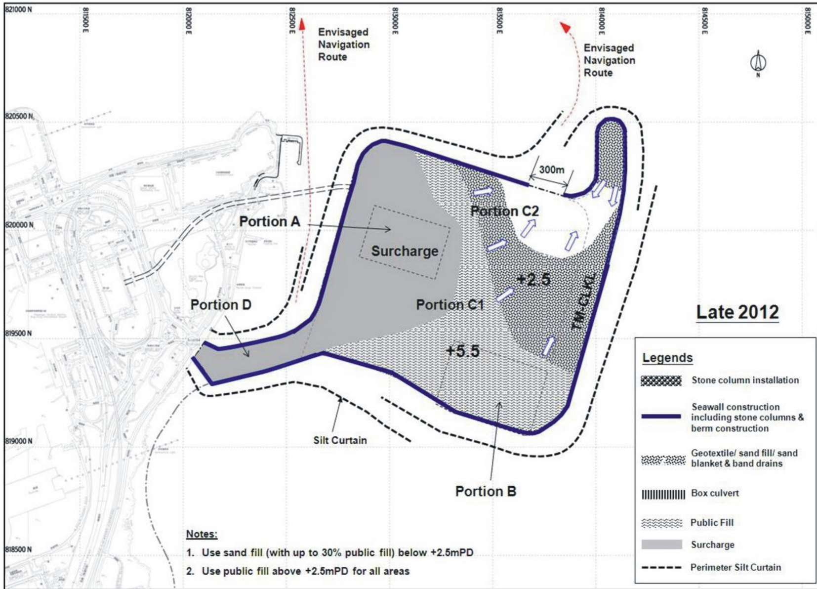
Figure 16 - Outline of Construction Sequence (Sheet 5 of 10) 圖 16 - 施工程序大綱(表10之5)
